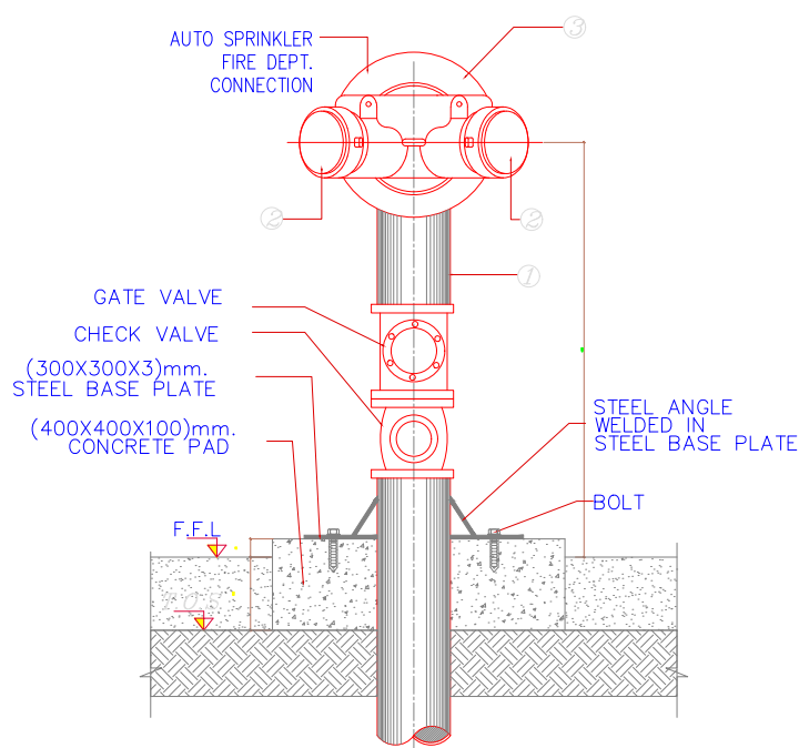
FIRE DEPARTMENT CONNECTION DETAIL
