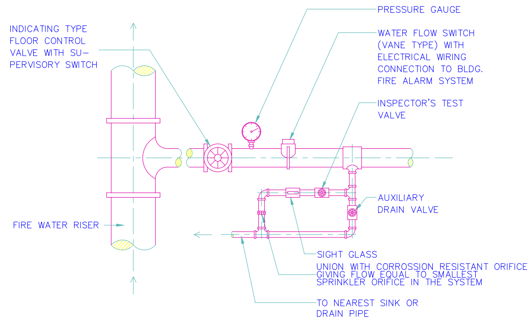
FLOOR CONTROL VALVE ASSEMBLY
