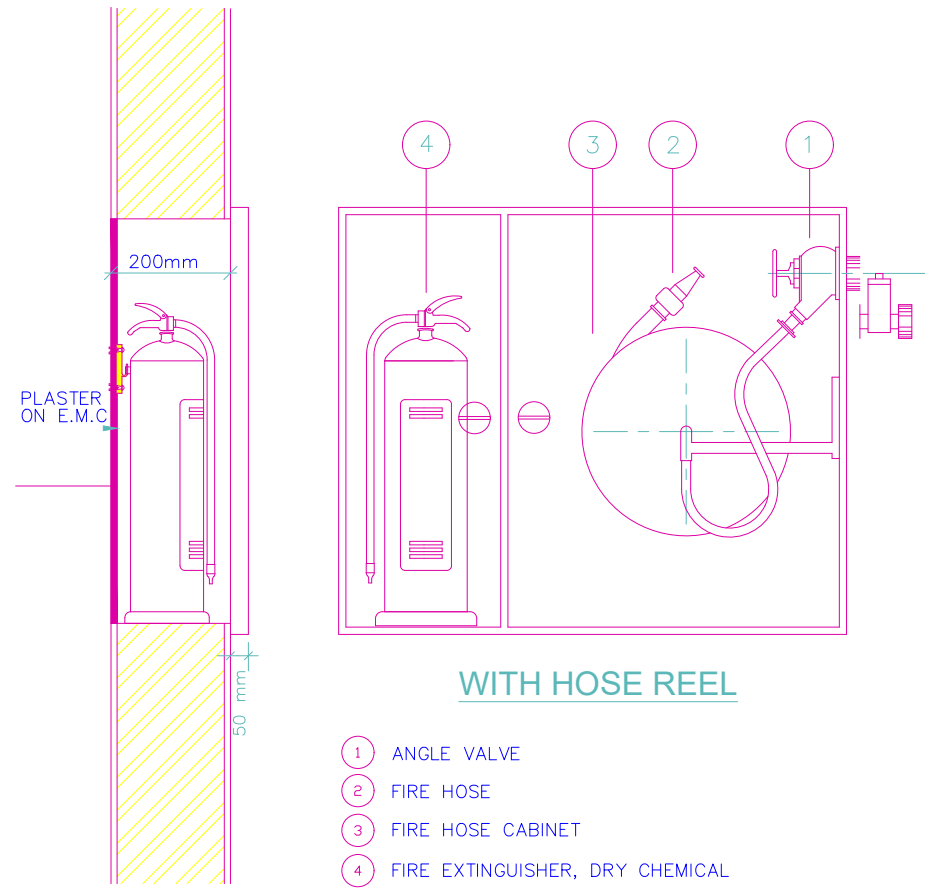
FIRE HOSE CABINET WITH EXTINGUISHER
