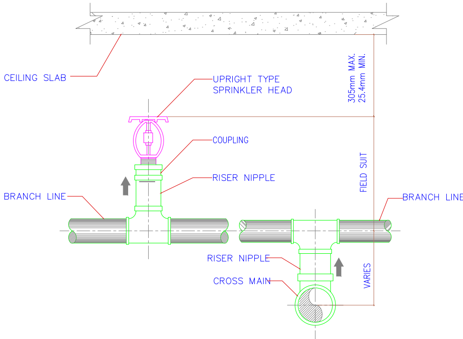
UPRIGHT TYPE SPRINKLER DETAIL
